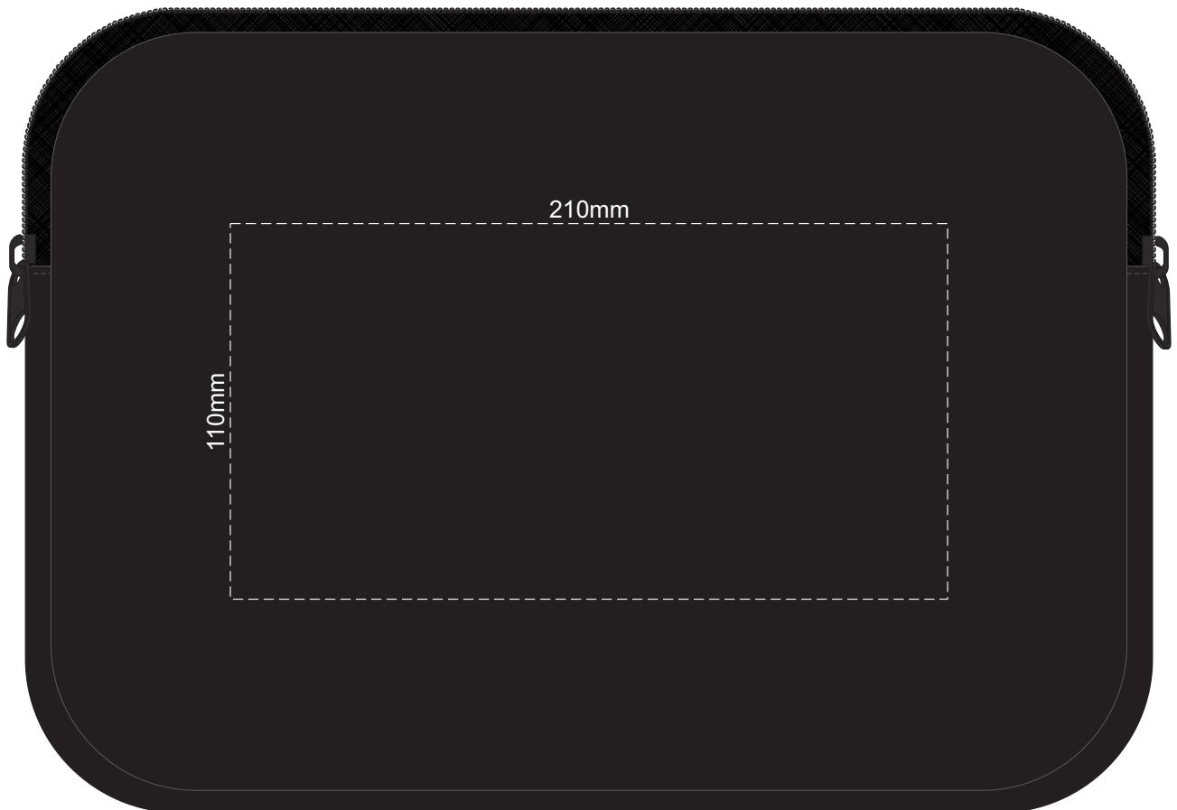
SIDE 2
